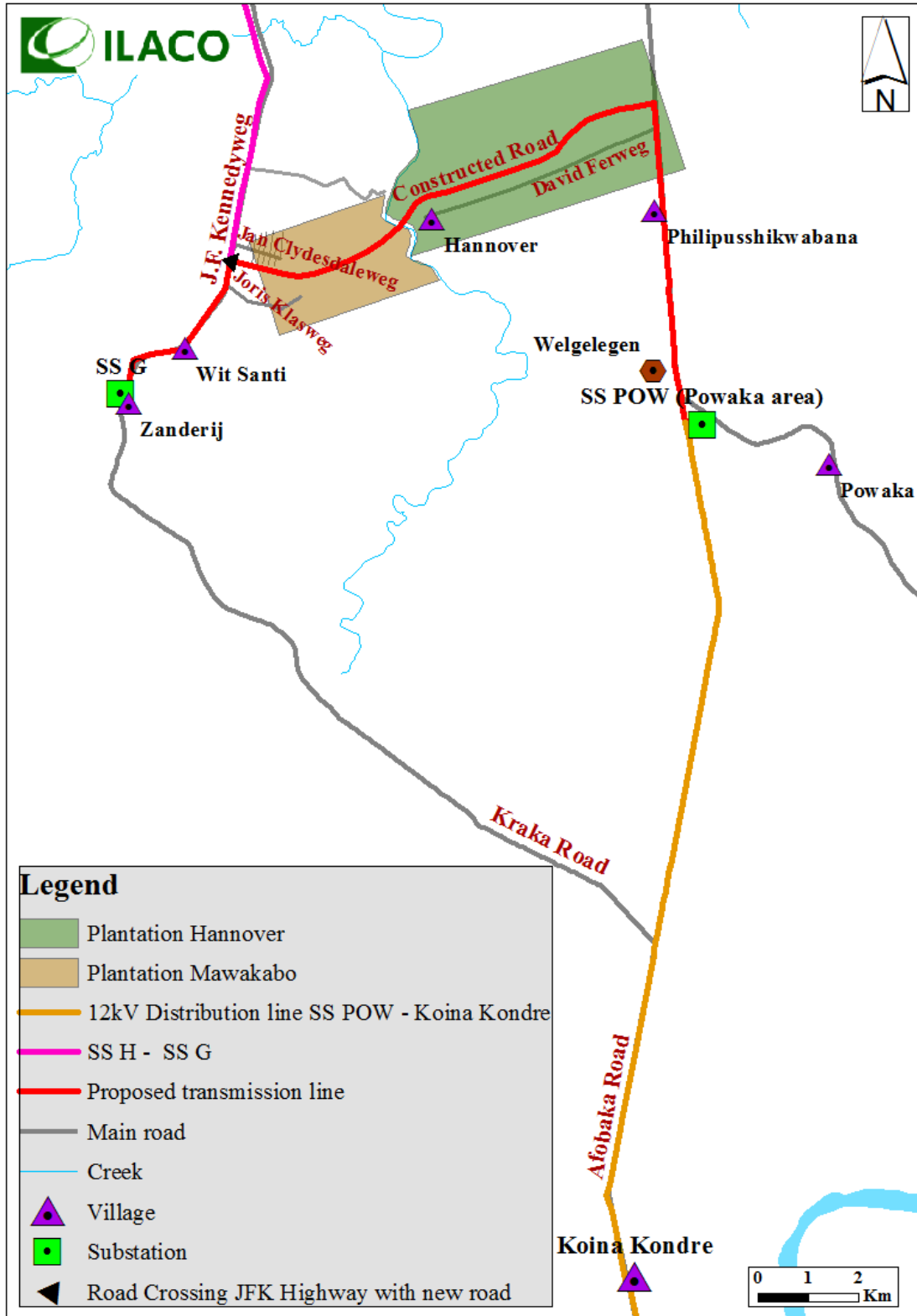
Figure 2: Overview Powaka - Zanderij transmission line project
