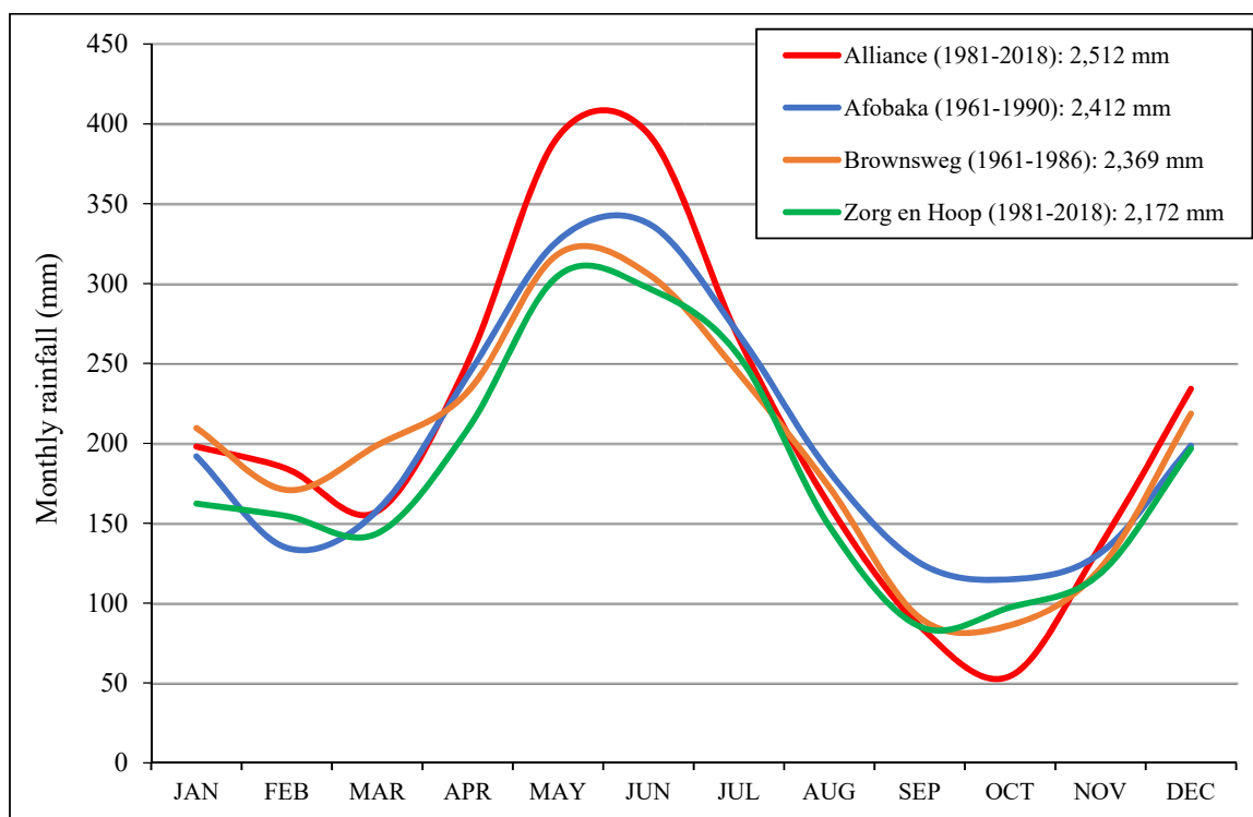
Figure 8: Long-term mean monthly and total annual precipitation for regional stations.
